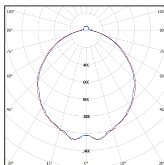
MXL1083 60W
