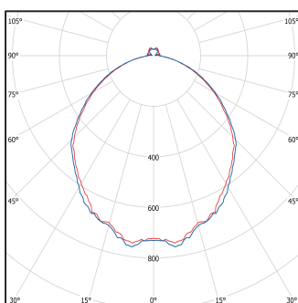
MXL1083 30W
